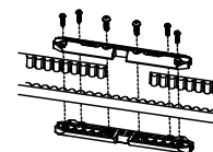
041A4021R Trolley latch (belt)
